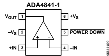
Figure 3. 6-Lead SOT-23 (RJ)
