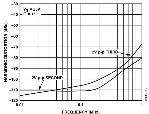
Figure 4. Harmonic Distortion
